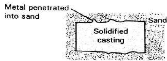
Figure 3.10 Penetration
