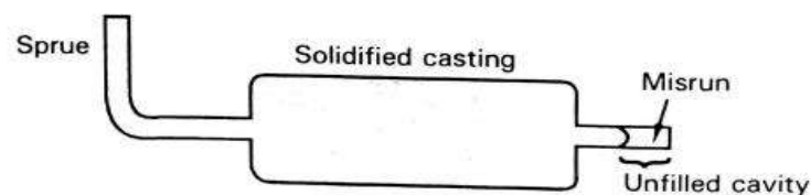
Figure 3.9 Misrun
