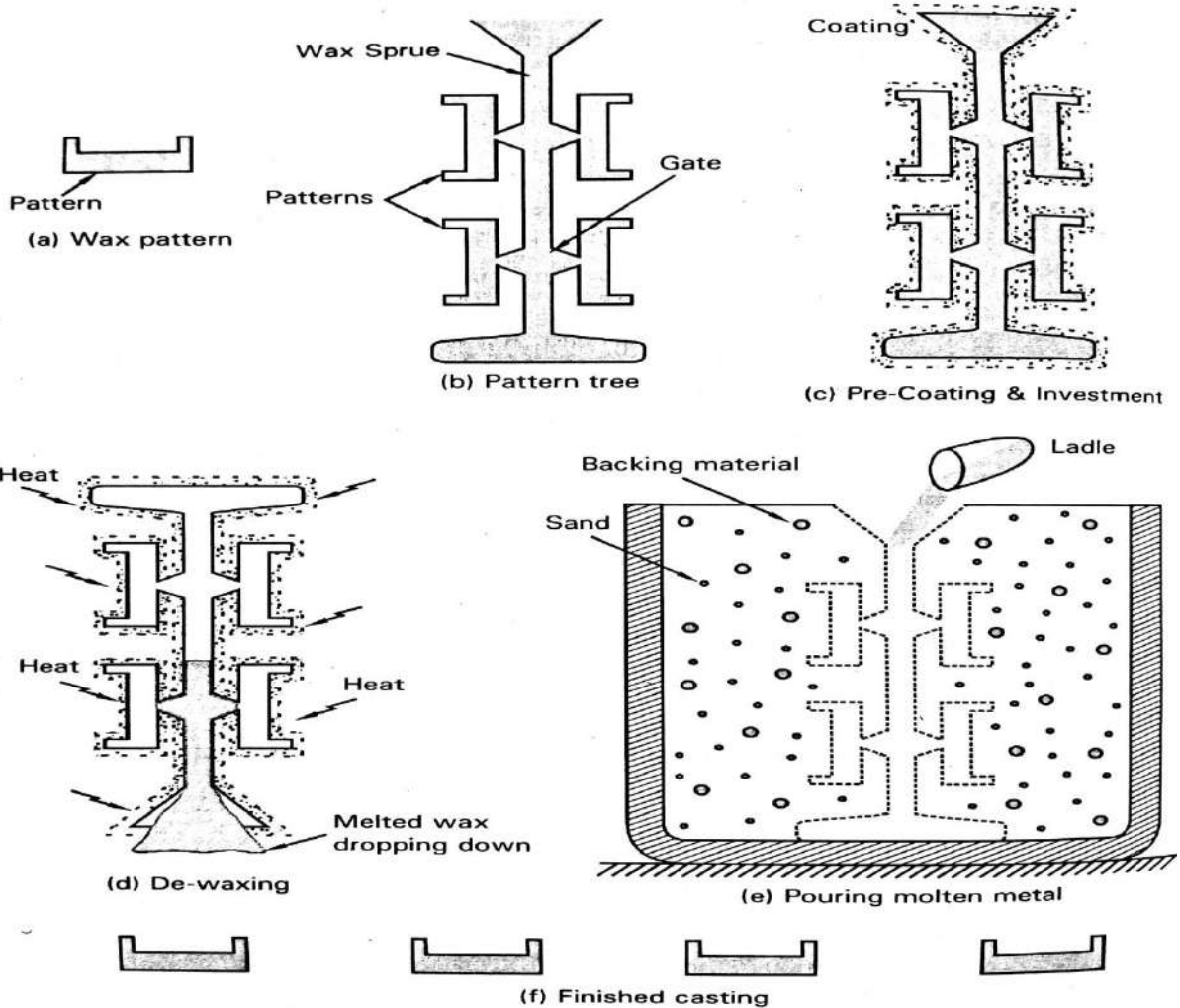
Investment moulding
