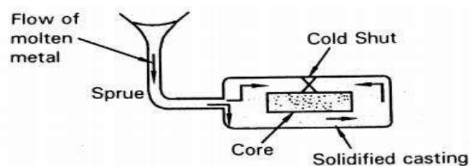
Figure 3.12 Cold shut
