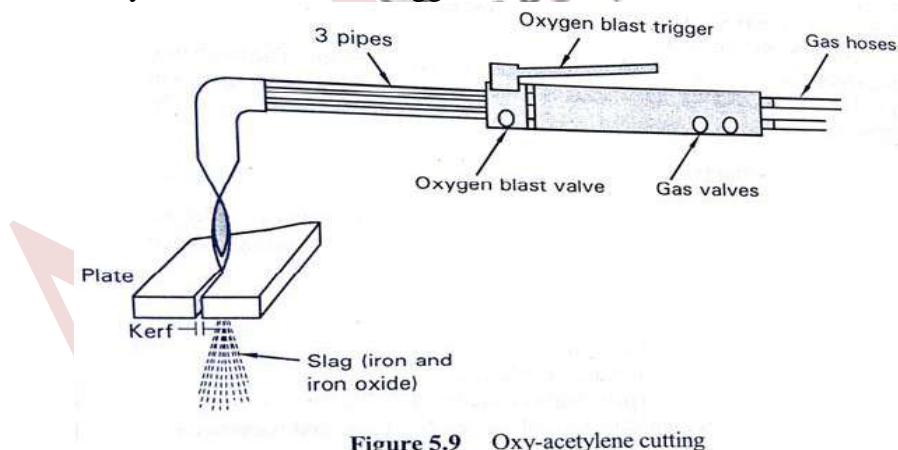
Figure 5.9 Oxy-acetylene cutting
