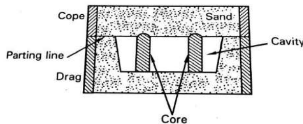
Kiss core
