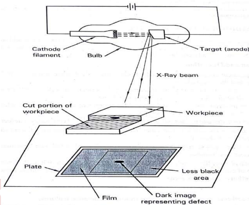
Figure 5.15 Radiography inspection
