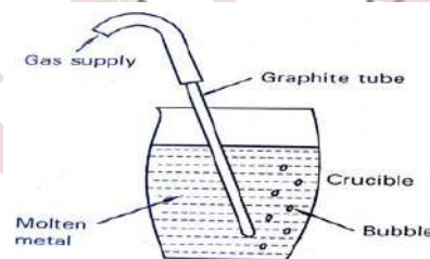
Figure 3.2 Flushing
