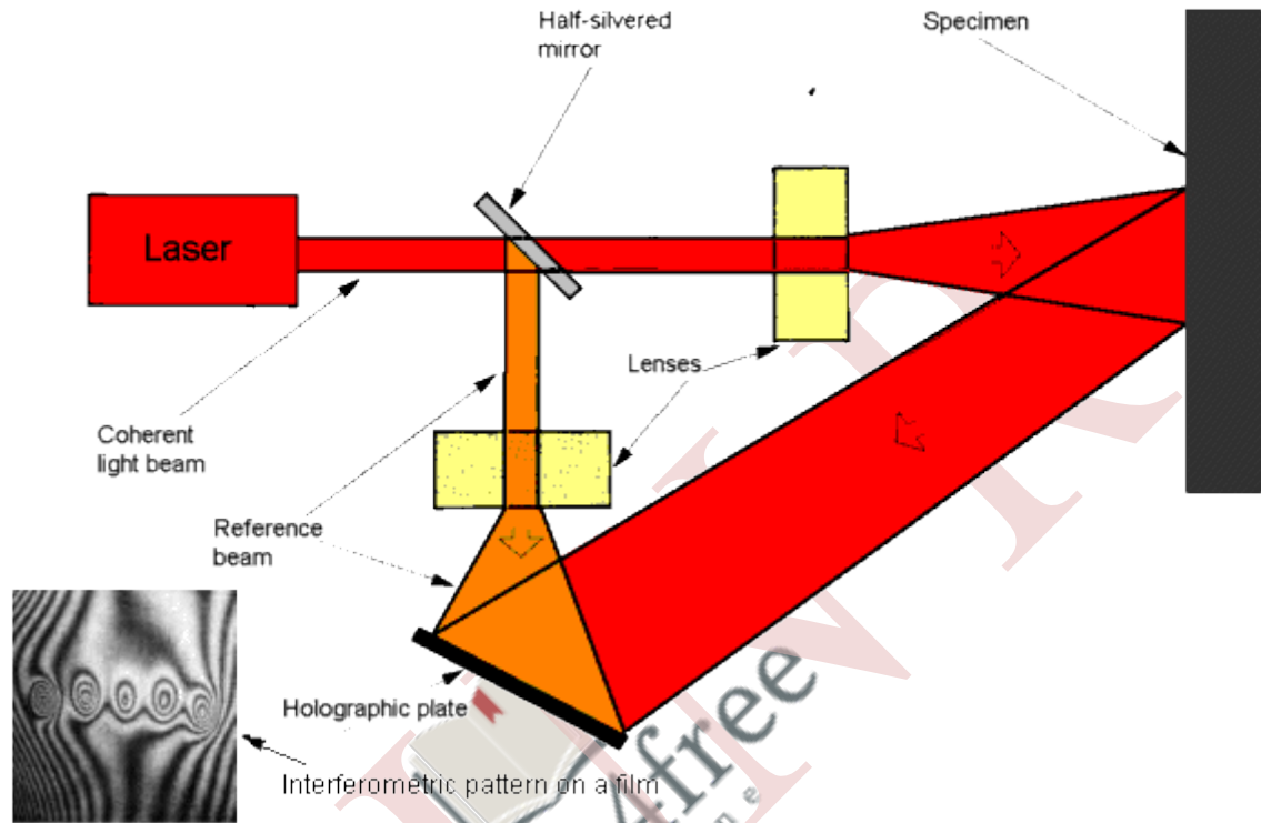
Figure 5.17 Holography Inspection
