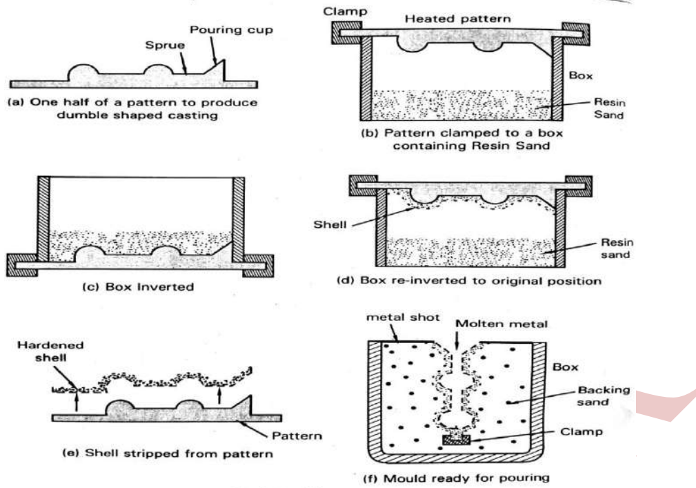
Shell Moulding
