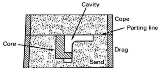
Drop core
